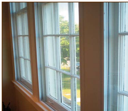
Climate Seal™ Acoustic Series window insert applied over historic wooden windows at the Mary O'Keefe Cultural Center. Ocean Springs, MS.
